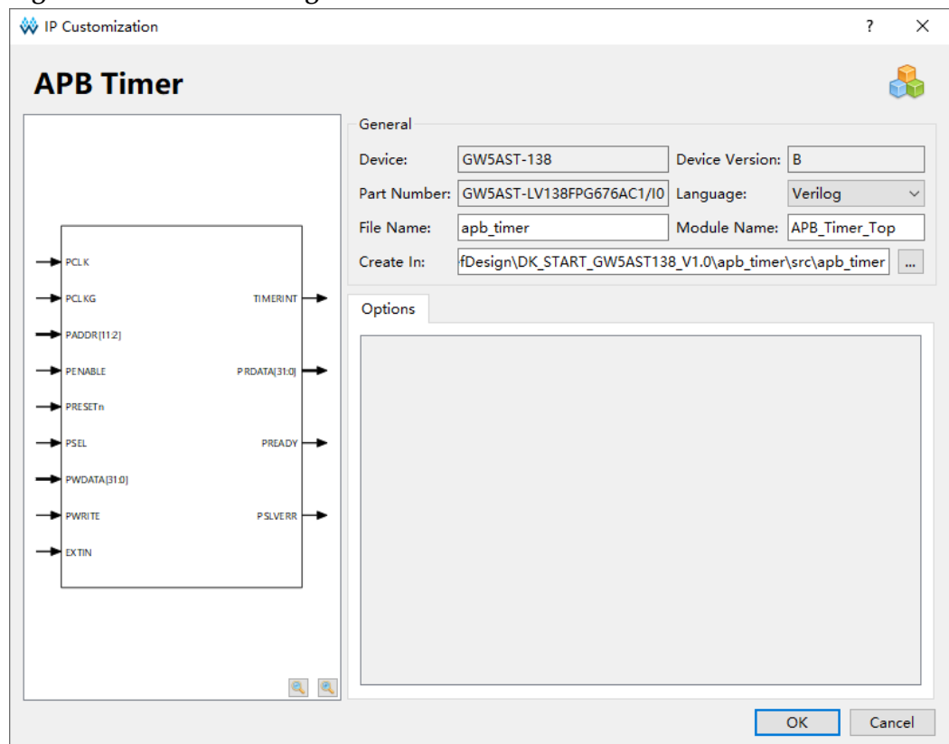
Figure 4-1 Interface Configuration
