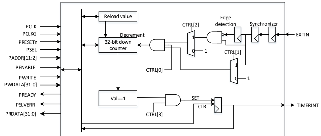
Figure 2-1 Structure Diagram
