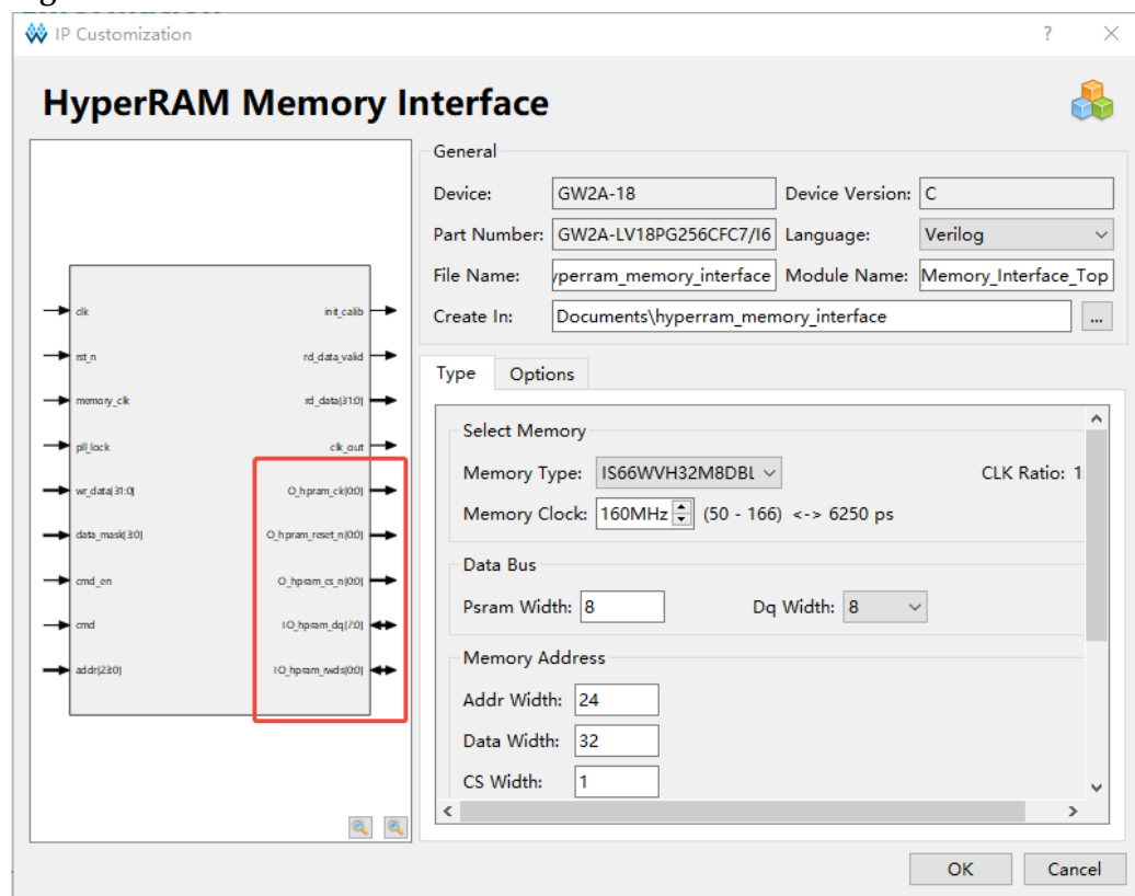
Figure 8-3 IP Core Interface
