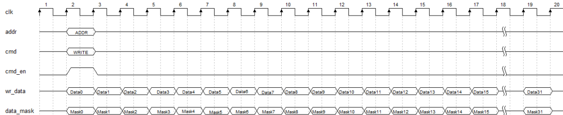
Figure 4-10 Write Data Timing with the Burst Length of 128
