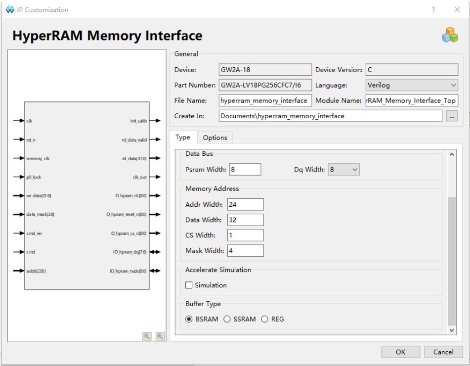
Figure 8-5 Configuration Interface
