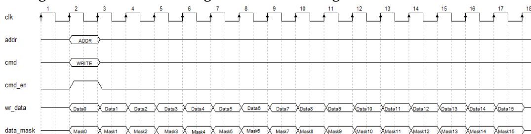
Figure 4-9 Write Data Timing with the Burst Length of 64
