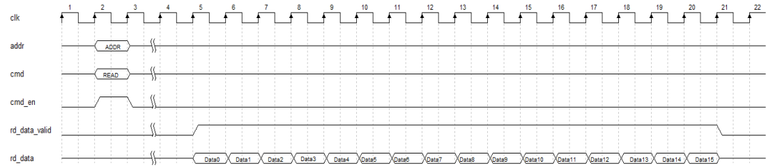
Figure 4-13 Read Data Timing with the Burst Length of 64
