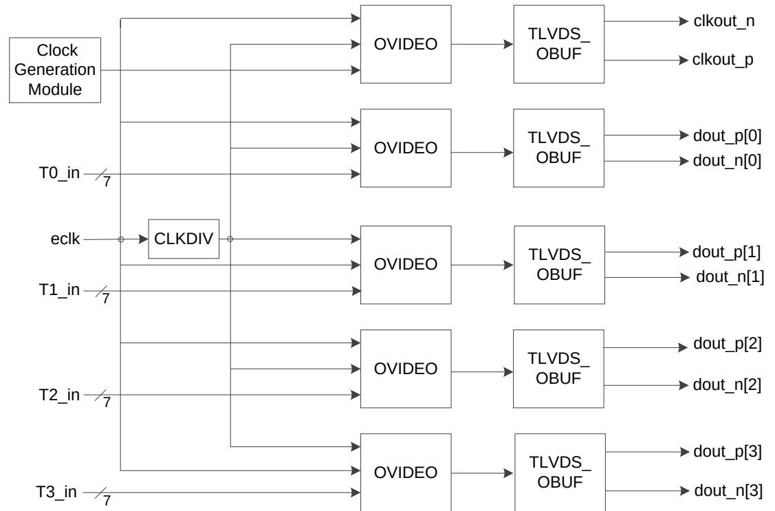
Figure 4-2: Functional Diagram of LVDS 7:1 TX Module
